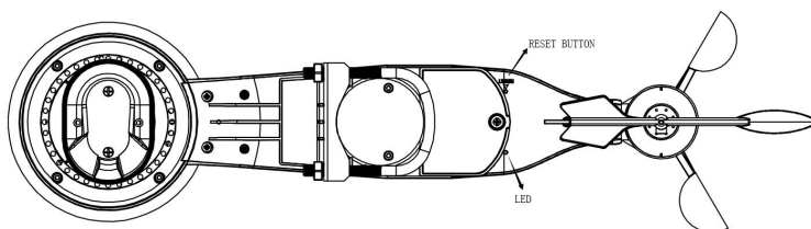
Figure 13 Reset button and Transmitter LED location
