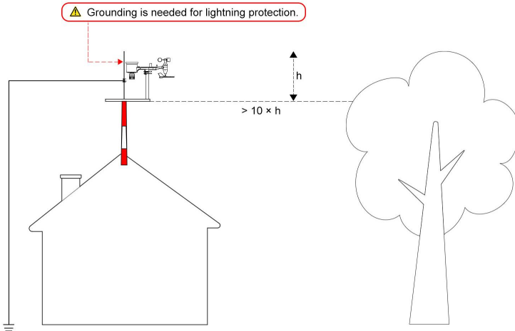
Figure 9 Grounding protection
