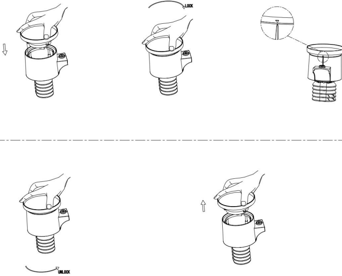
Figure 11 Rain gauge installation and maintenance
